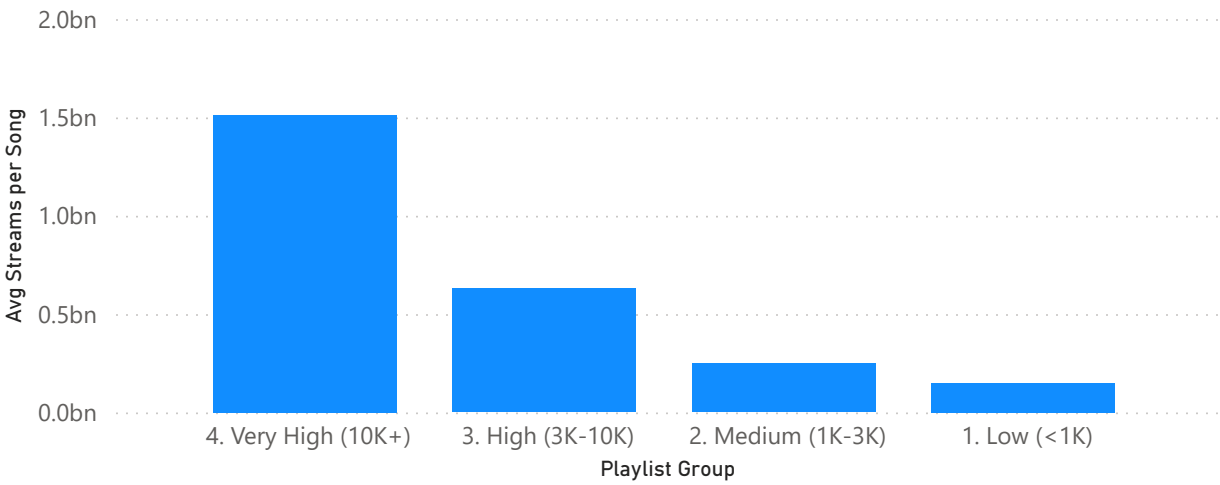
Avg Streams per Song by Playlist Group
